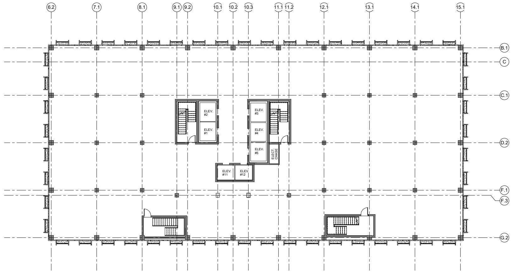
① 34TH FLOOR NOT TO SCALE
