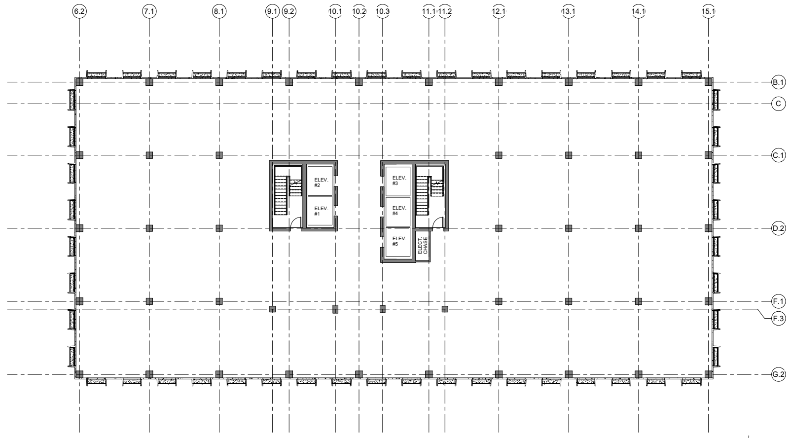
1 25 THRU 32 TYPICAL FLOOR PLAN NOT TO SCALE
