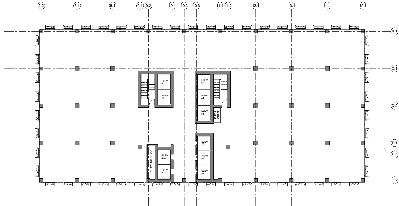
① 9 THRU 21 TYPICAL FLOOR PLAN NOT TO SCALE
