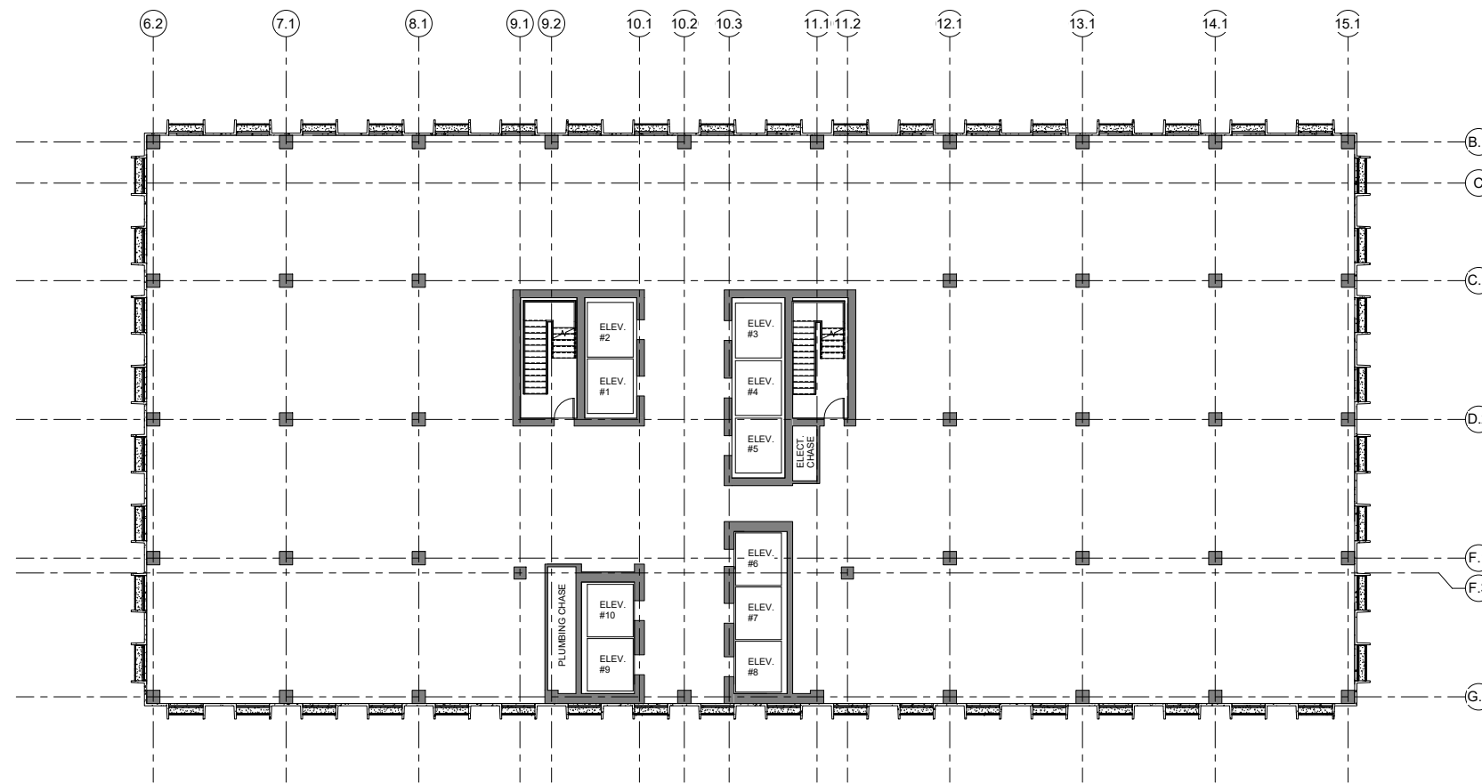
② 22ND FLOOR NOT TO SCALE
