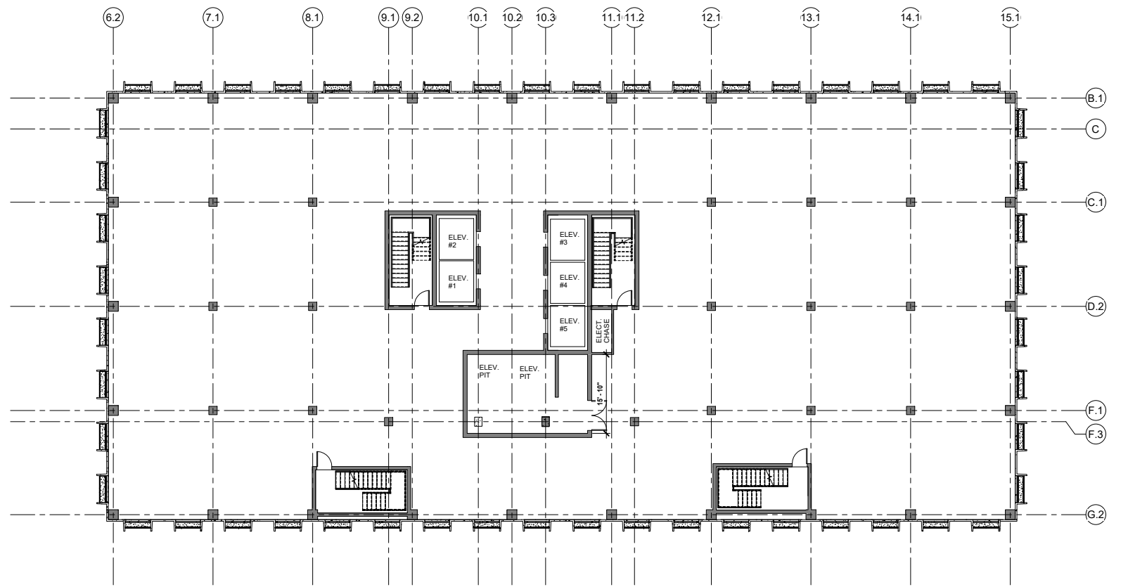
2 33RD FLOOR PLAN NOT TO SCALE
